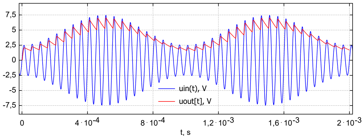
Amplitude detector
